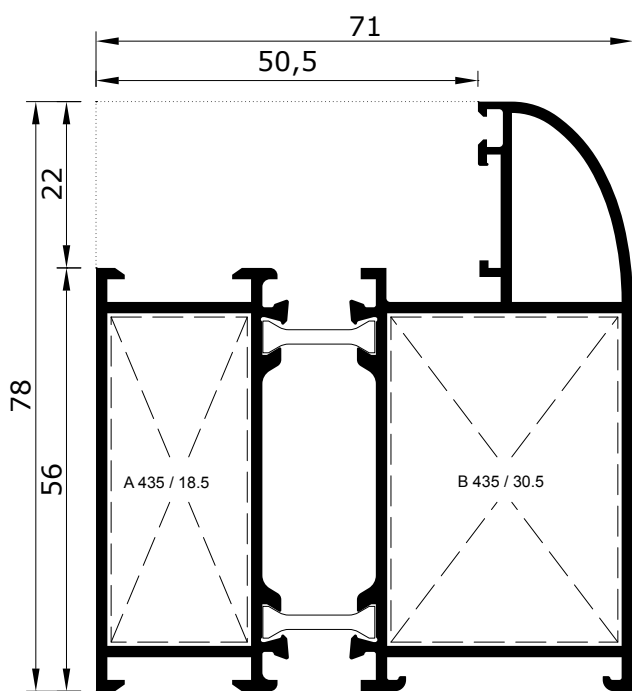
EX-55 14078-15
