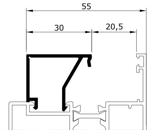
EX 50030-15 0.367 kg/m
