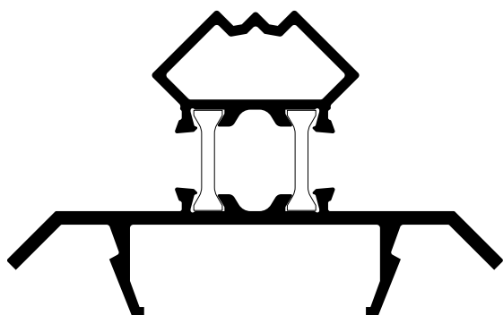
EX-55 40100-15
