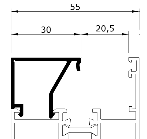
EX 50030-15 0.367 kg/m
