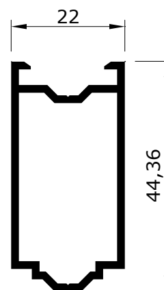
EX-55 42040-15
