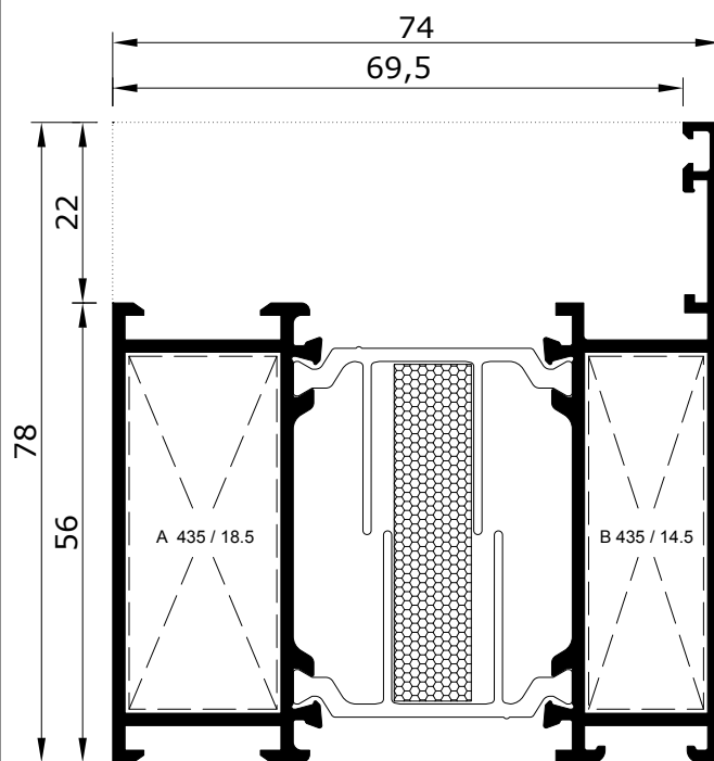
EX-74 10078-15
