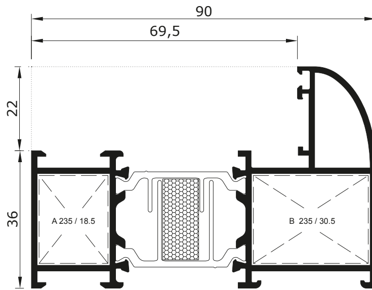
EX-74 14058-15
