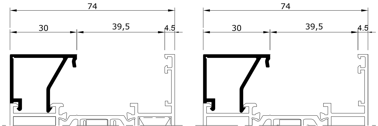
EX 50030-15 0.367 kg/m
