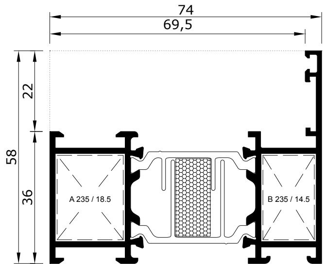
EX-74 10058-15
